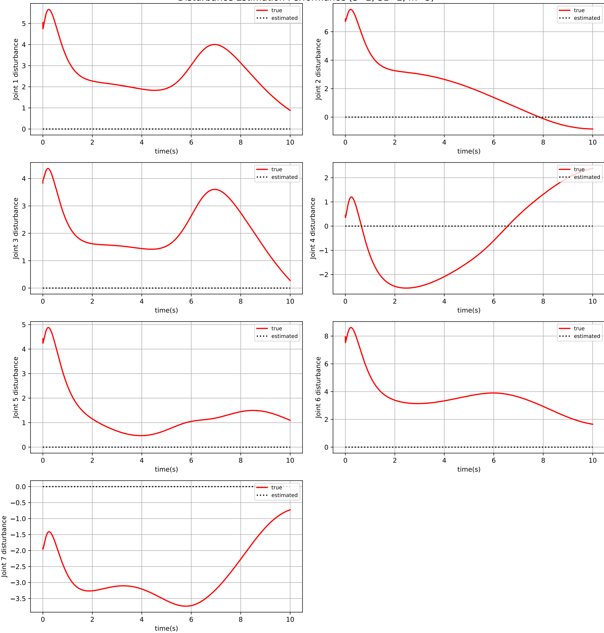
Disturbance Estimation Performance (S=2, S1=2, m=5)
